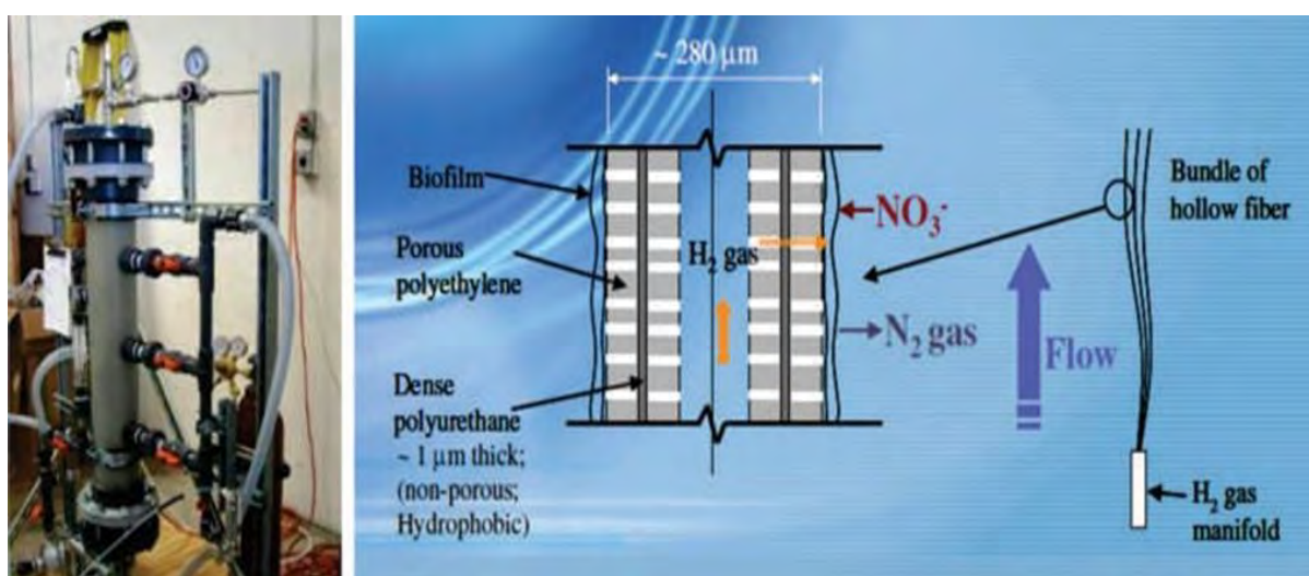
Figure 31: Advanced Nitrate Reduction Hollow Fiber Membrane Reactor (Source: Hand Book for Drinking Water Treatment, JJM, Ministry of Jal Shakti, Gov. of India)
